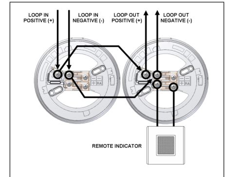
Figure 2 - adaptor base and deep adaptor base loop wiring.
